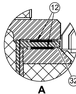
F-231 MK2-L CONFIGURATION MK2 PLUG SHOWN
